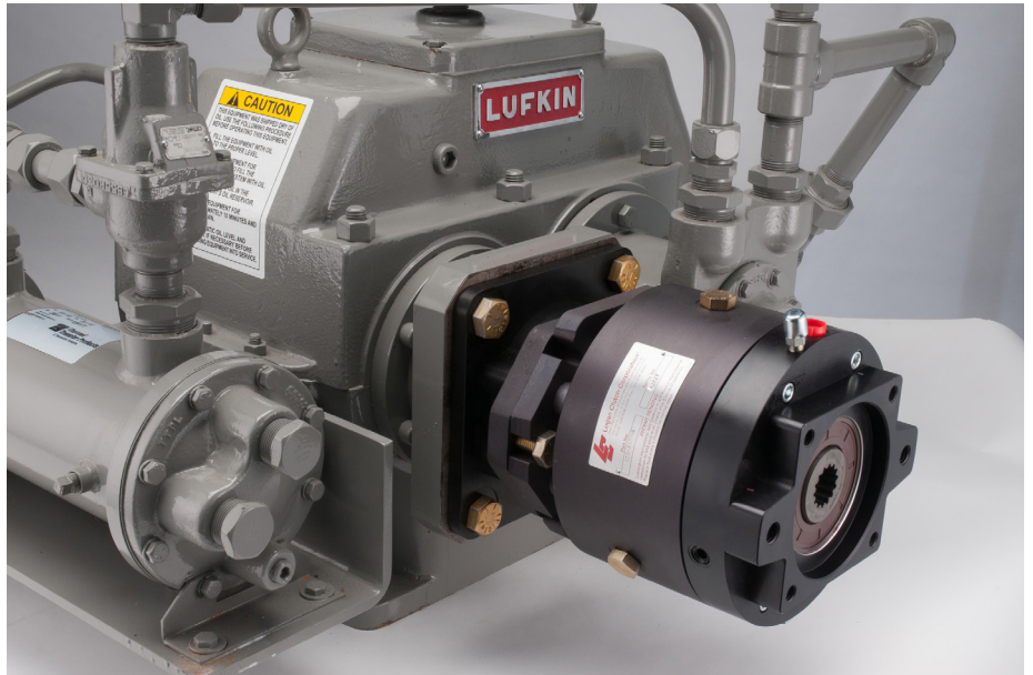
Lufkin Gearbox with Logan 600 Series Direct Drive PTO (600 lb. ft. / 1335 Nm) @ 200 psi. / 13.6 bar. The Logan PTO is positioned between a pump and gearbox, enabling power on demand for cold starts, and connect-disconnect applications.
