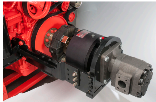
Logan Front PTO's act as connect/ disconnect for auxiliary pumps
