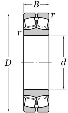
Cylindrical Bore
